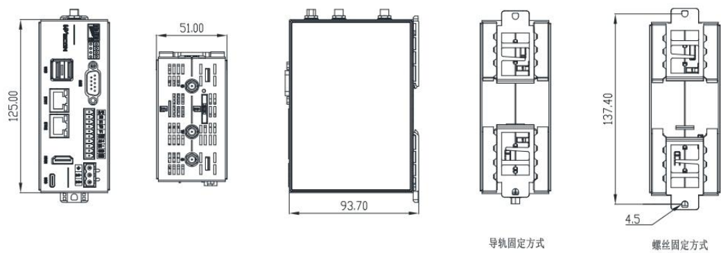
RH-00/RH-W/RH-G/RH-AG/RH-WG 安装尺寸图
