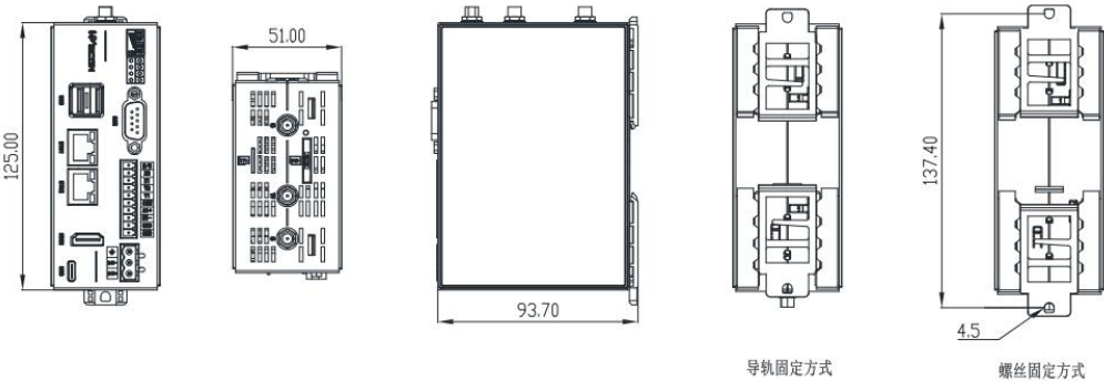
RH-00/RH-W/RH-G/RH-AG/RH-WG 安装尺寸图
